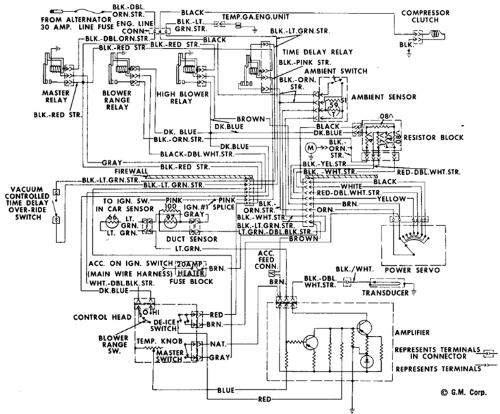
1968 Pontiac Automatic Temperature Control A/C & Heat
