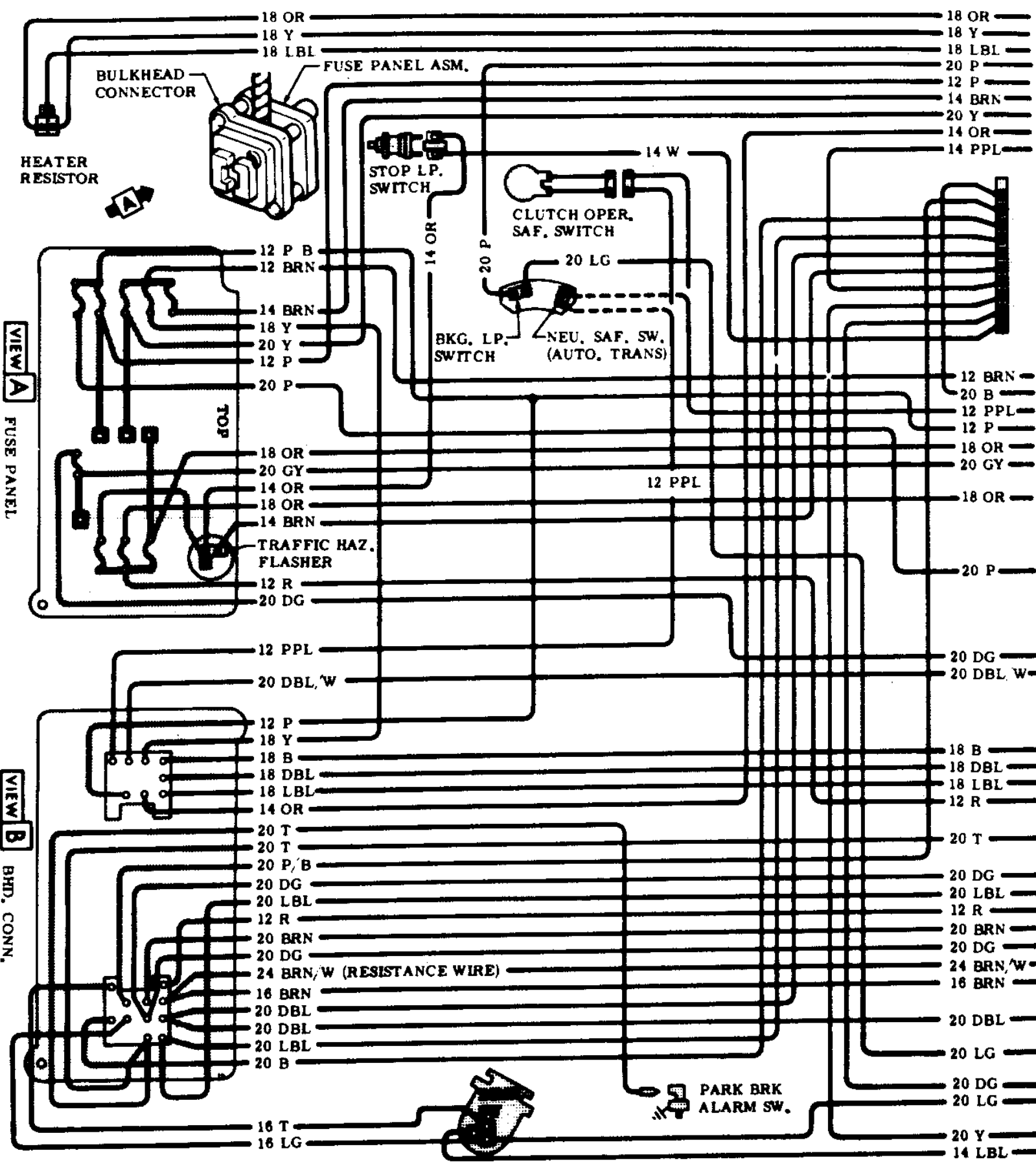
1969 Chevy II & Nova Fuse Panel
