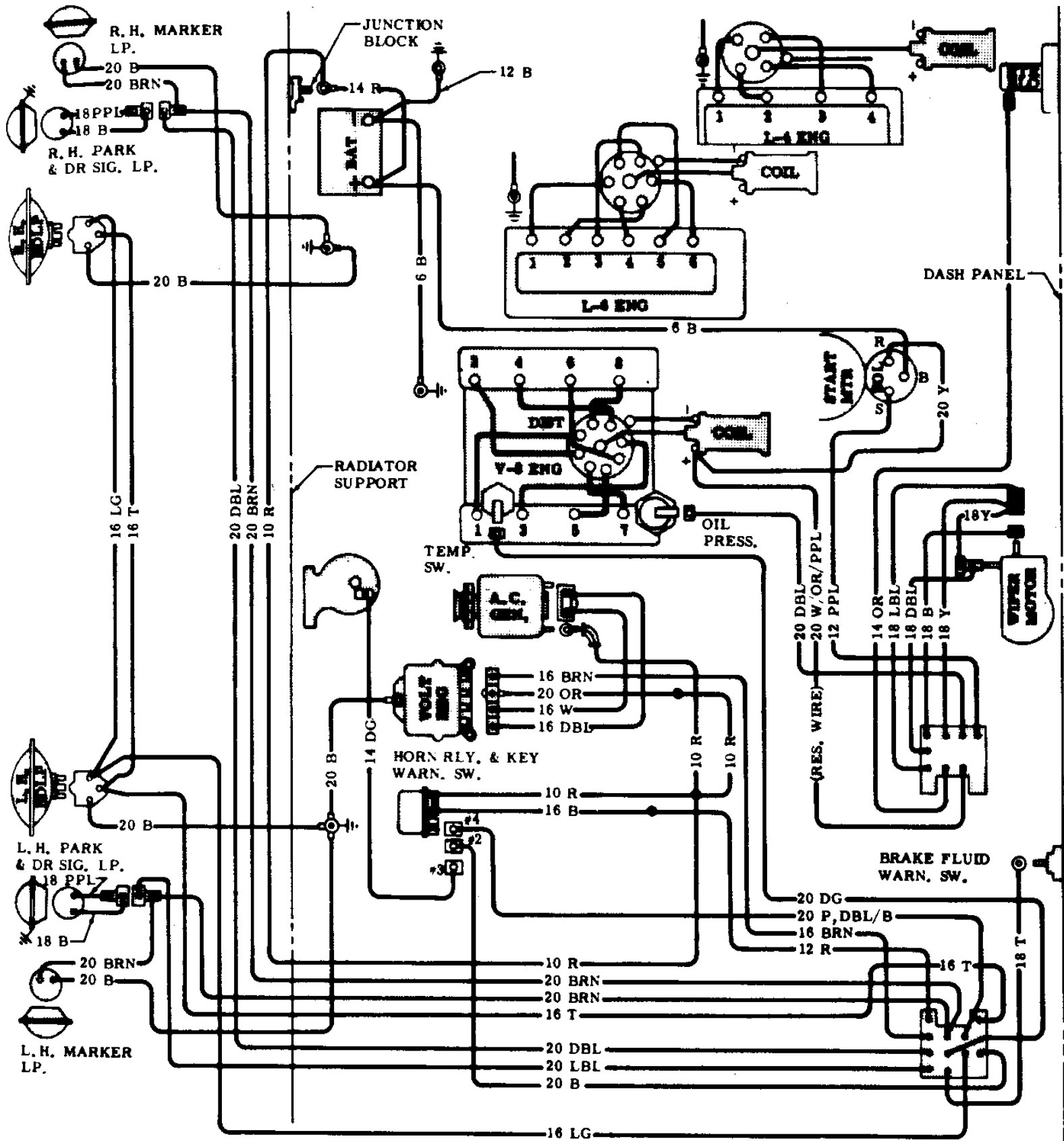
1969 Chevy II & Nova Front Lights & Engine
