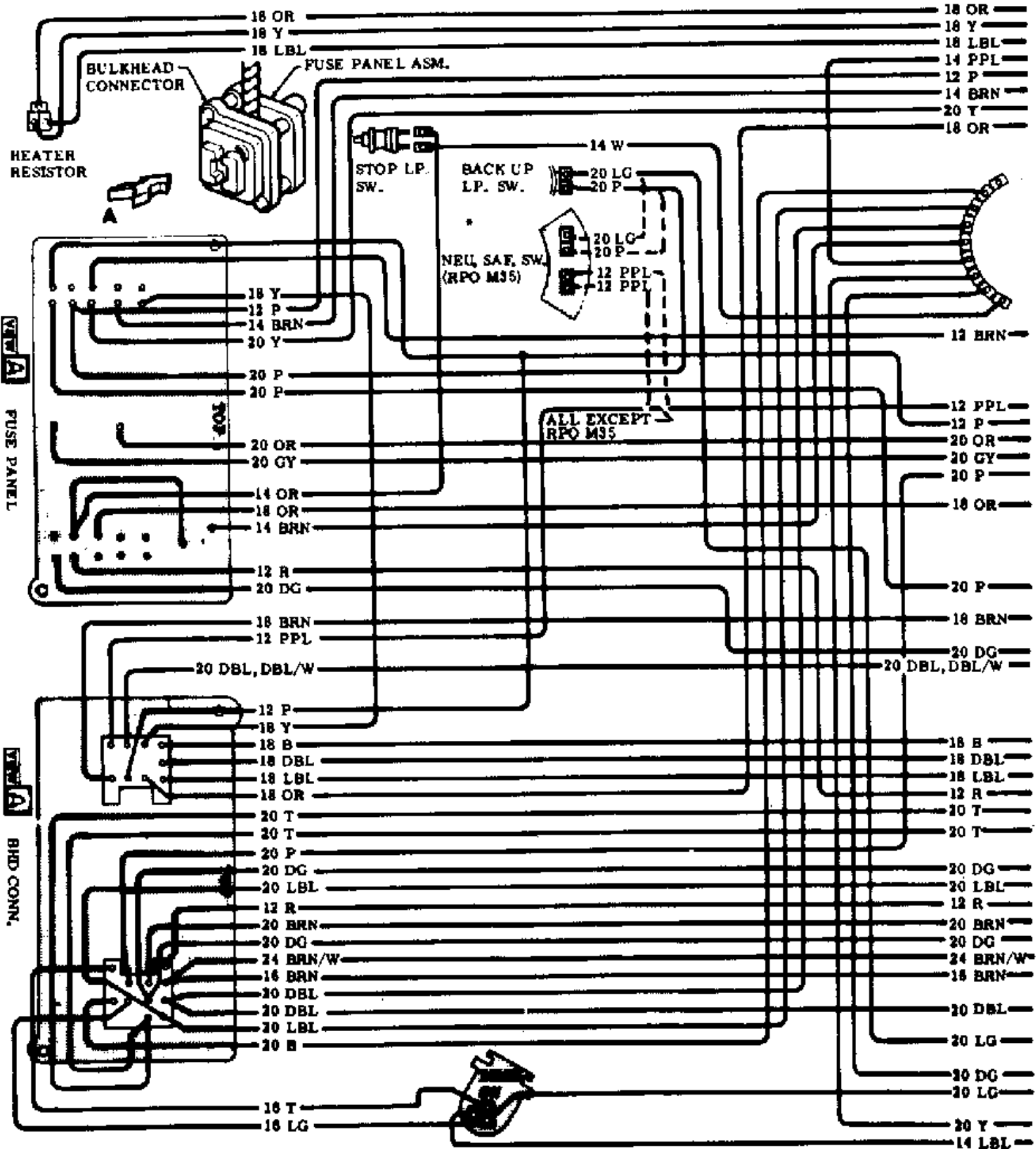
1968 Nova Fuse Panel
