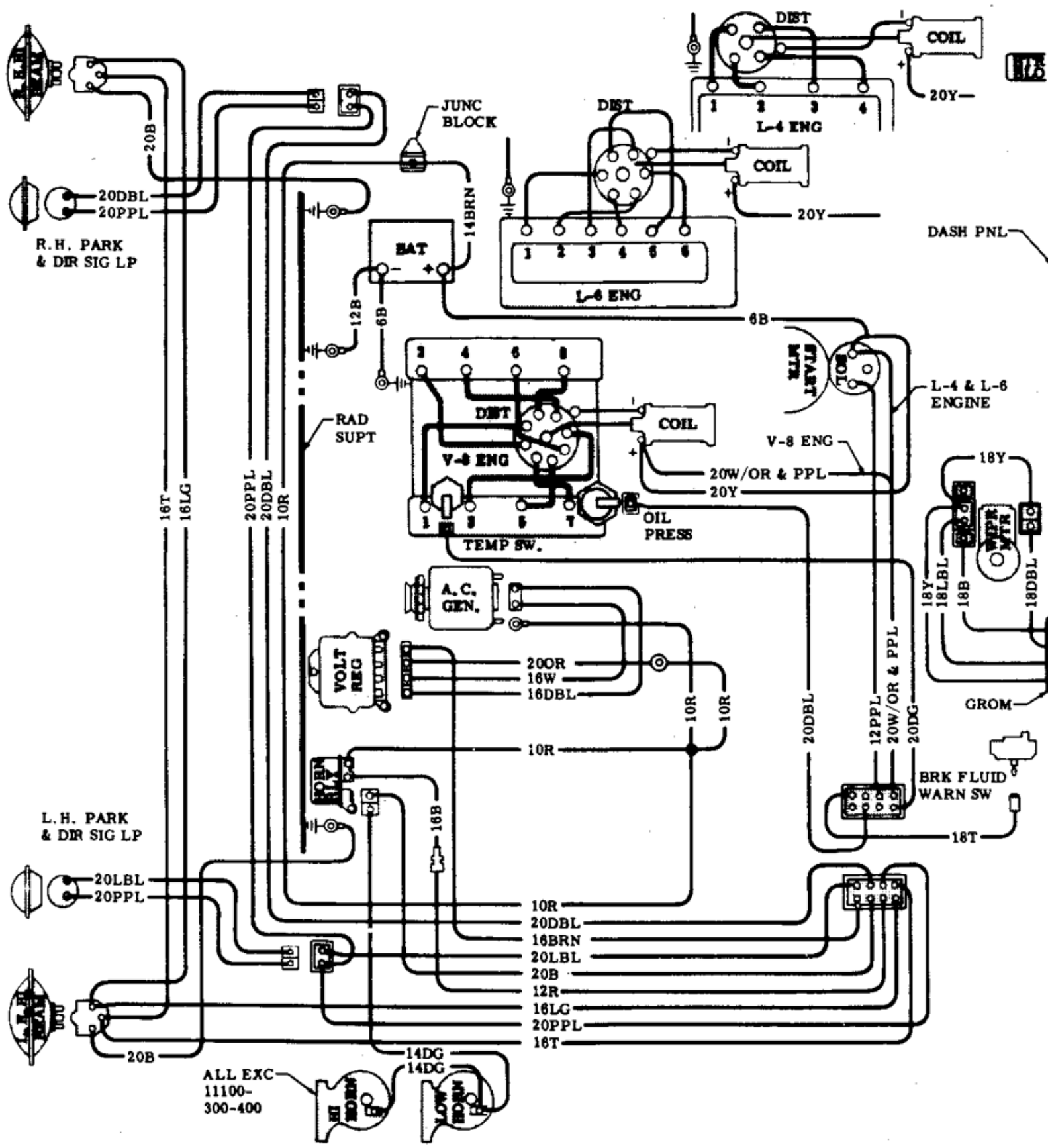
1967 Nova Front Lights & Engine
