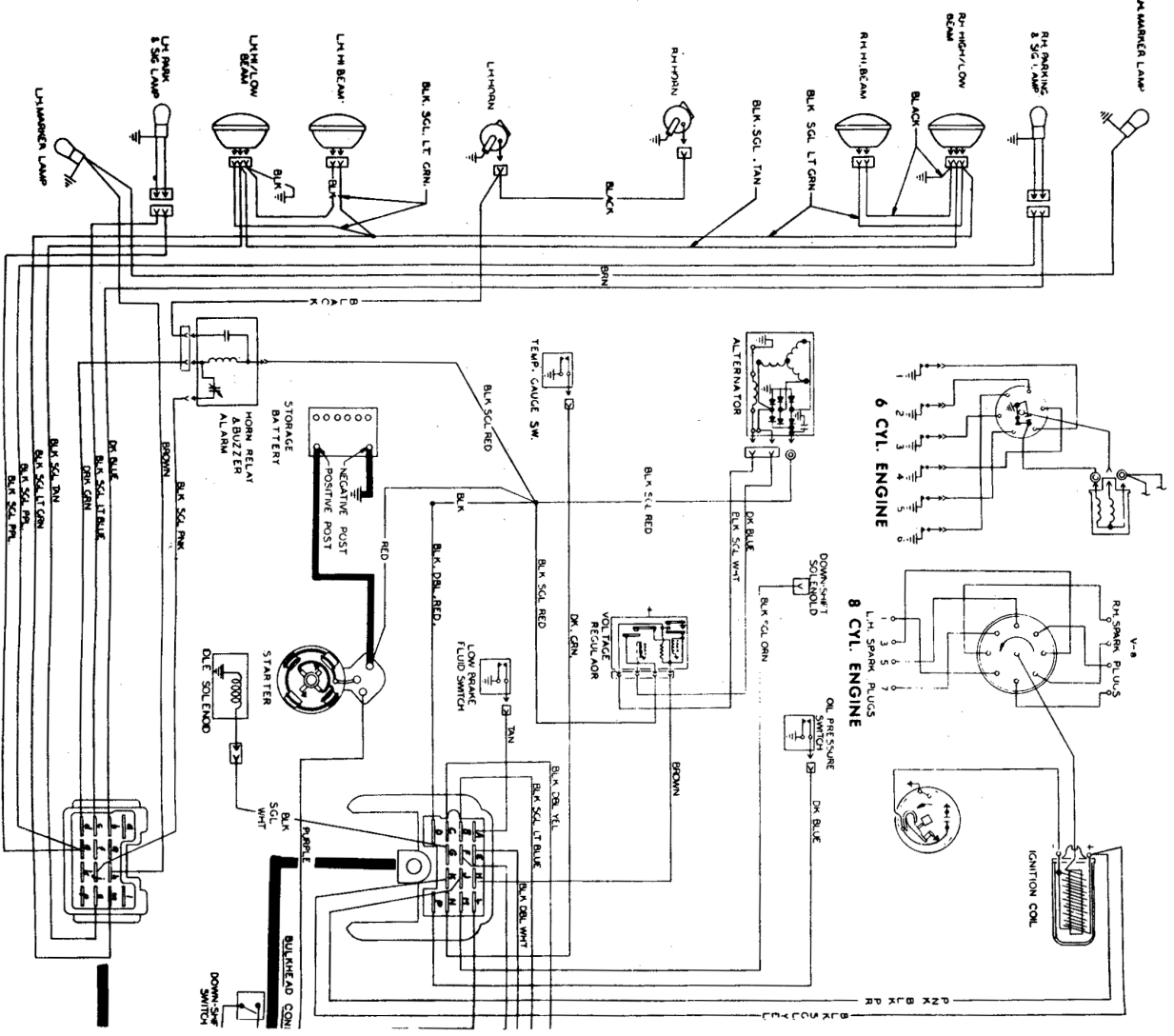
1967 GTO, LeMans & Tempest Chassis Wiring Diagram (FRONT HALF)
