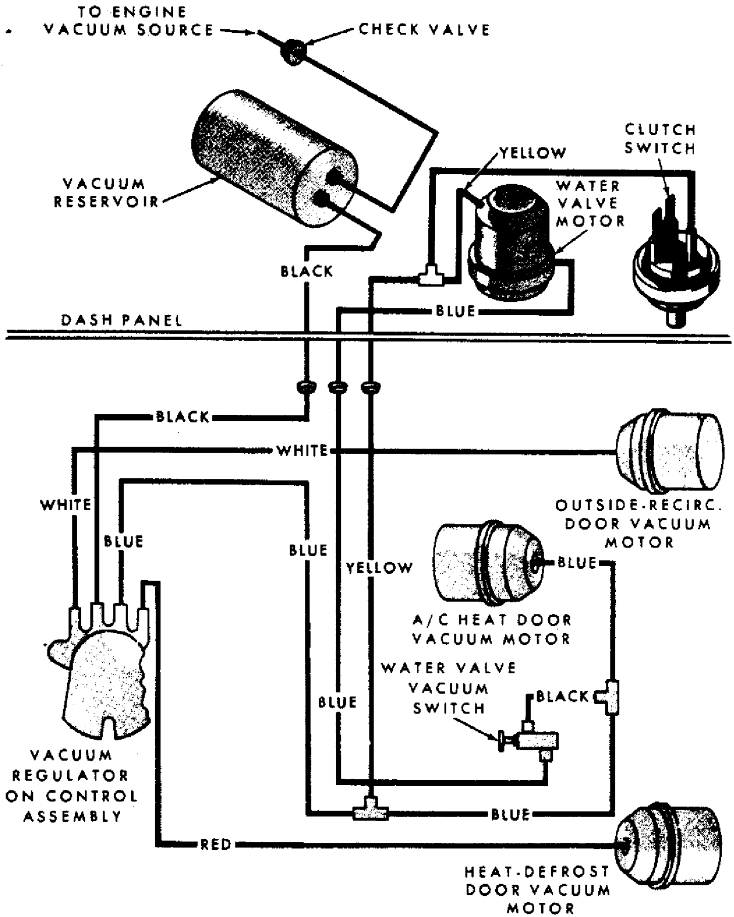
1969 Falcon & Fairlane A/C Heater Vacuum Circuit
