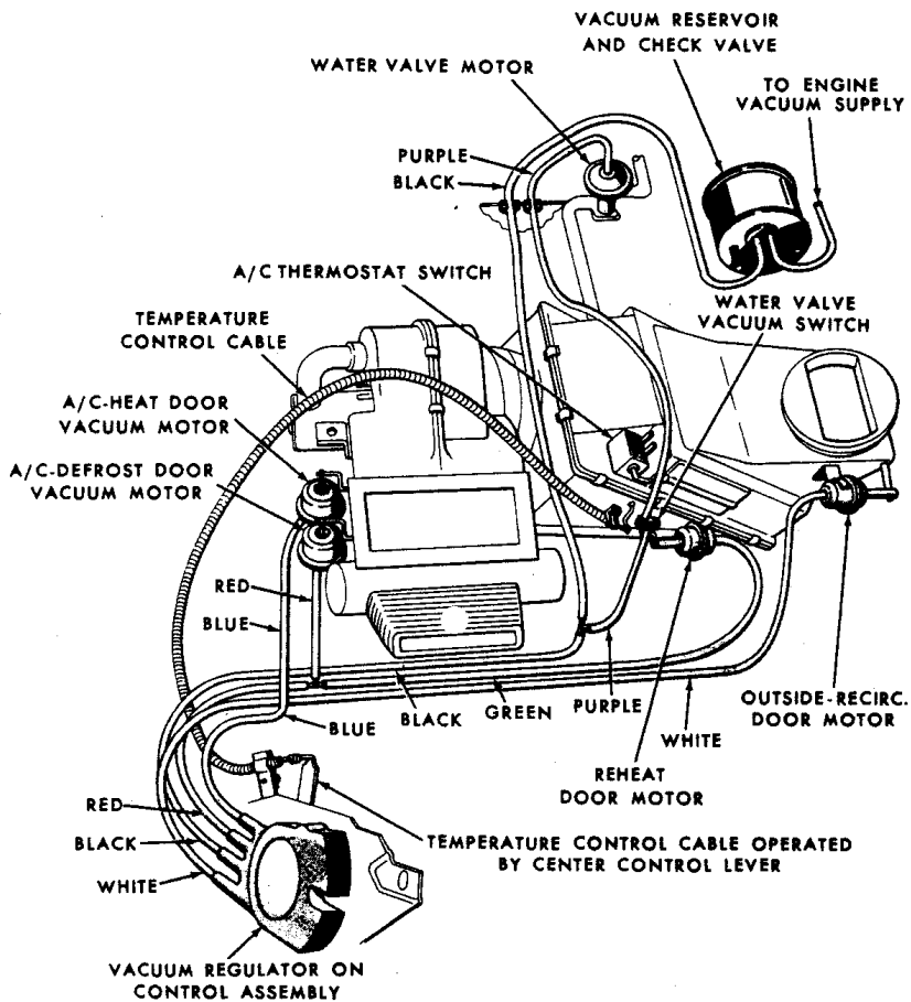
1967 (late) to 1968 Mustang & Cougar A/C Heater Vacuum Circuit
