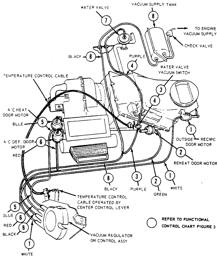
1967 (early) Mustang & Cougar A/C Heater Vacuum Circuit
