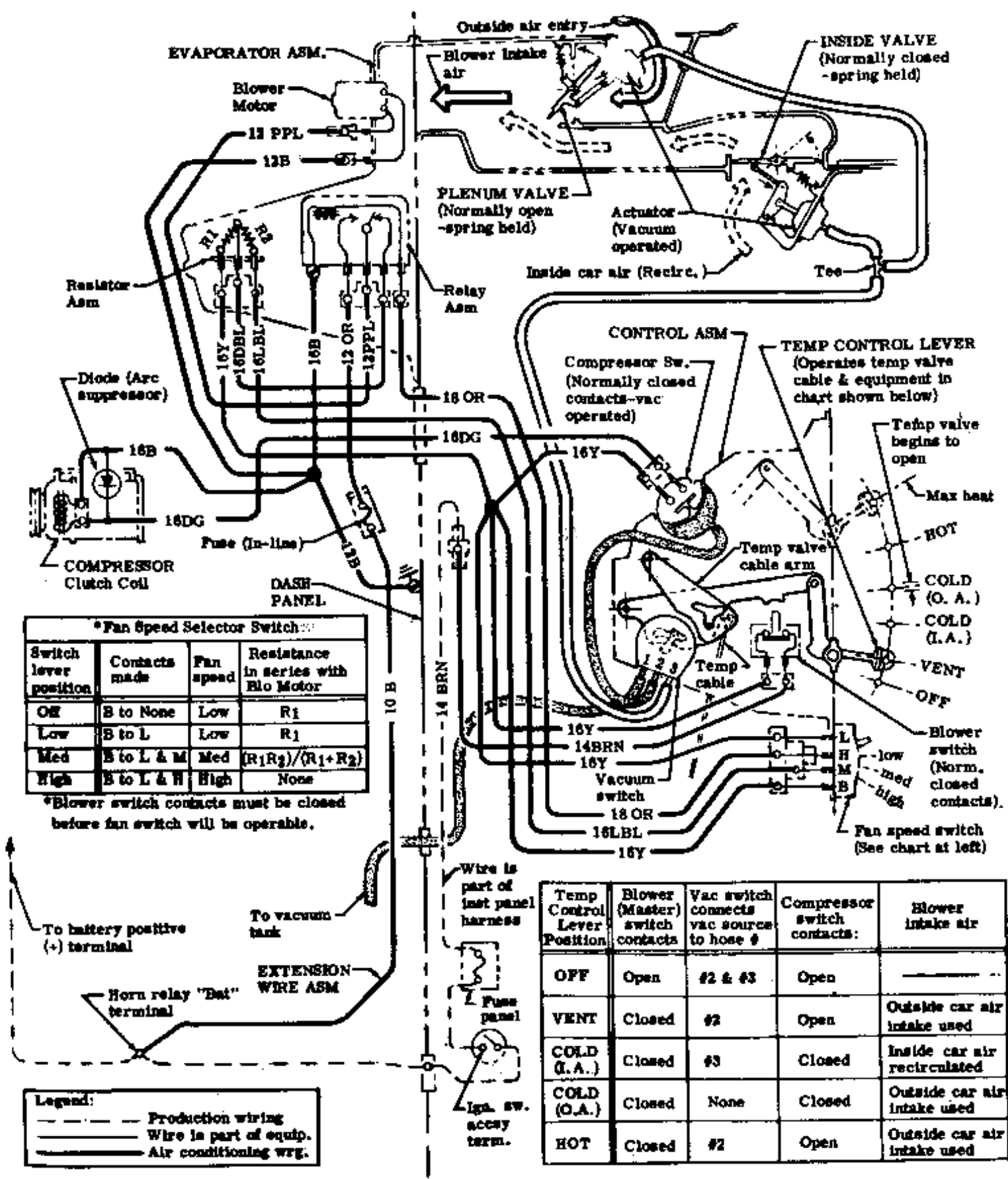
1967 FIREBIRD A/C & HEATING CIRCUIT
