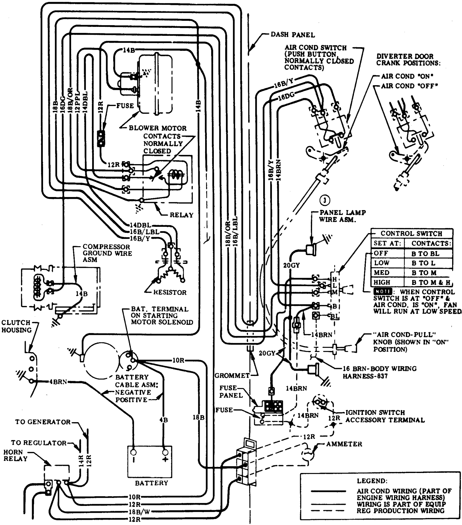
1967 Corvette A/C Heater Wiring Diagram
