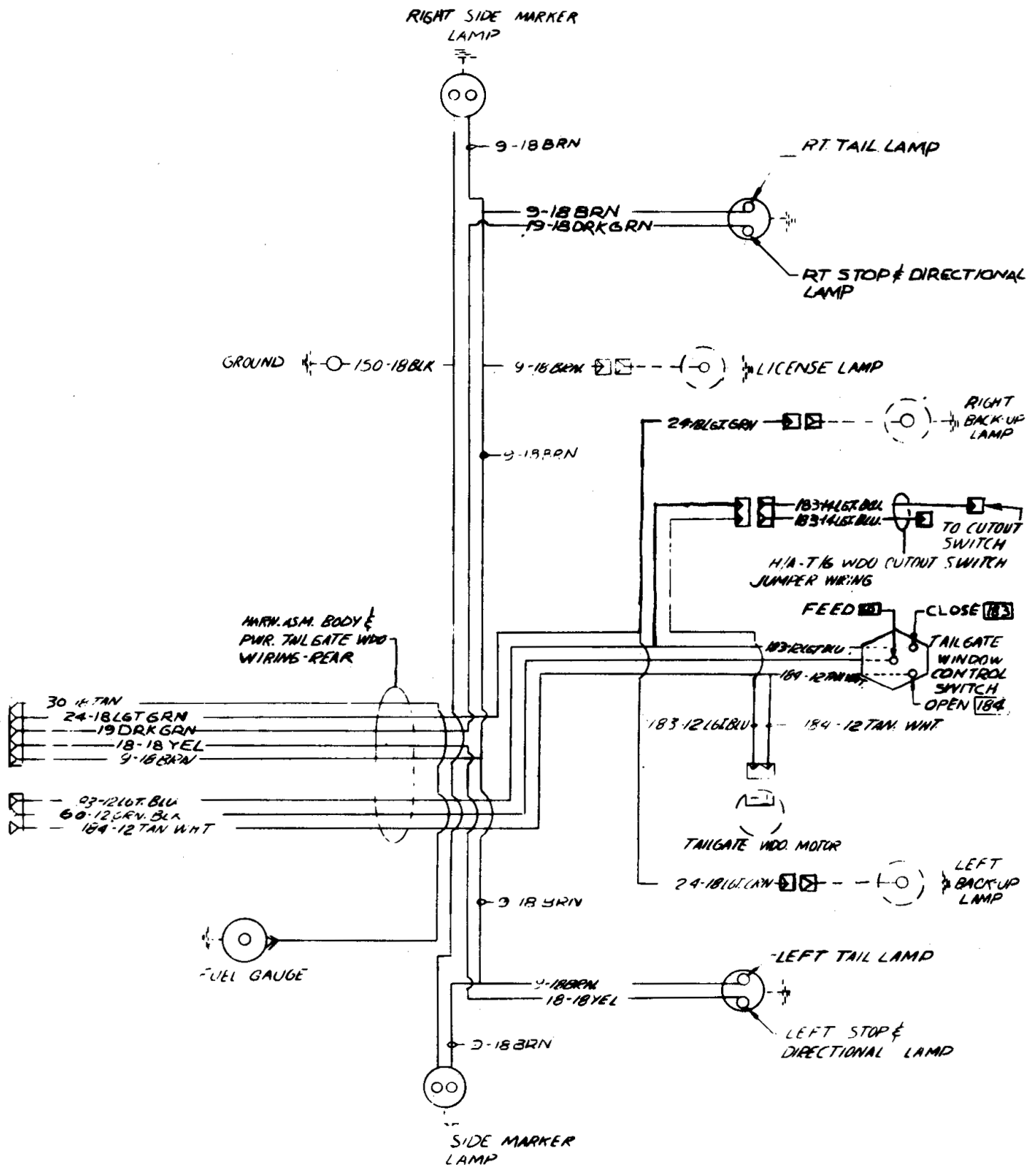
1971-72 Chevelle Wagon Power Tailgate Window Rear Circuit
