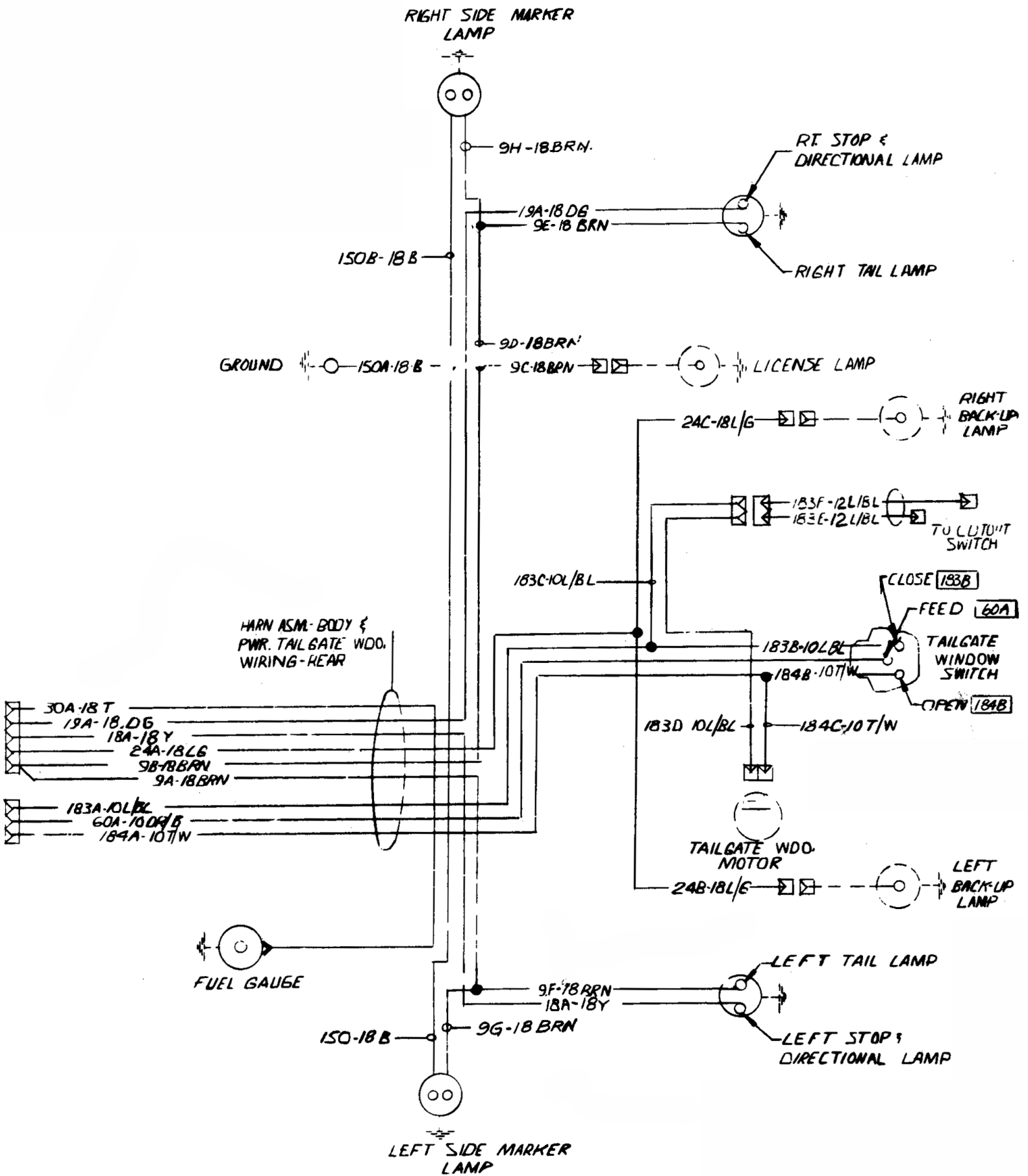
1970 Chevelle Wagon Power Tailgate Window Rear Circuit
