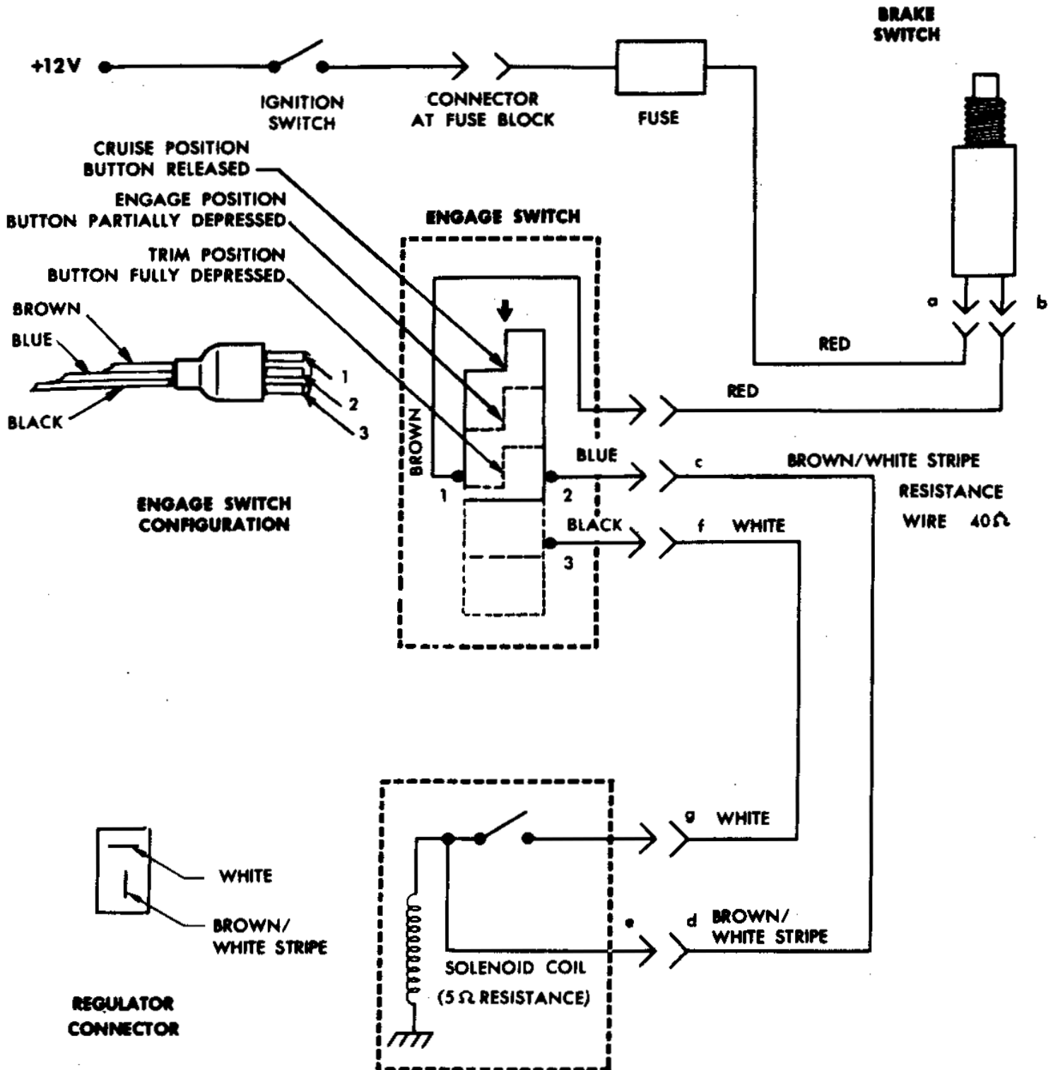
1970-72 Chevelle, El Camino & Monte Carlo Cruise Master Wiring Circuit
