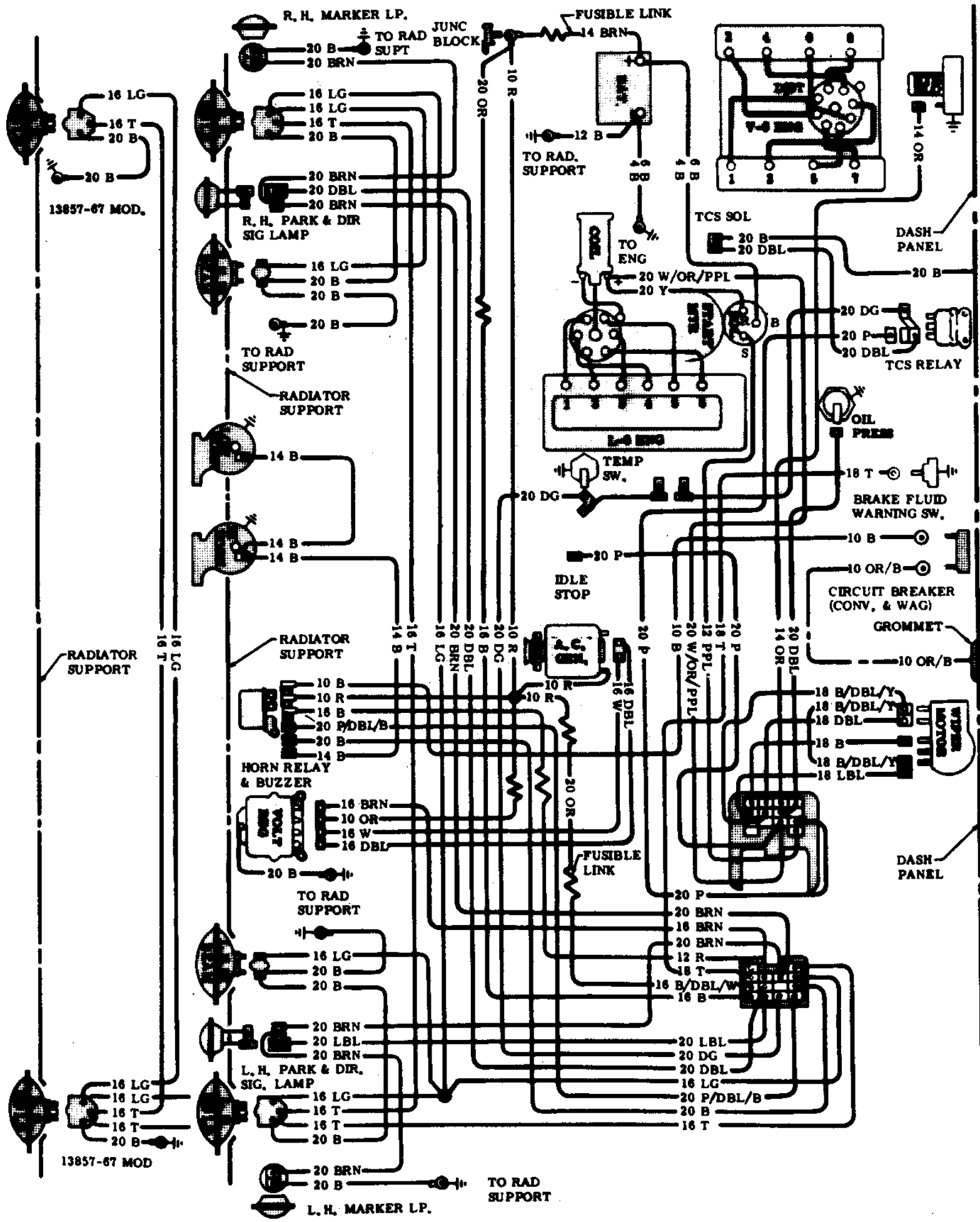
1970 Chevelle, El Camino & Monte Carlo Front Lights & Engine Diagram
