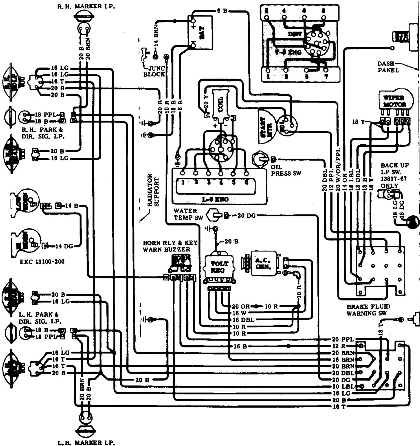
1968 Chevelle & El Camino Front Lights & Engine
