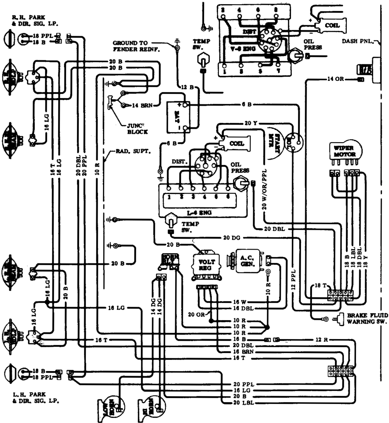
1967 Chevelle & El Camino Front Lights & Engine
