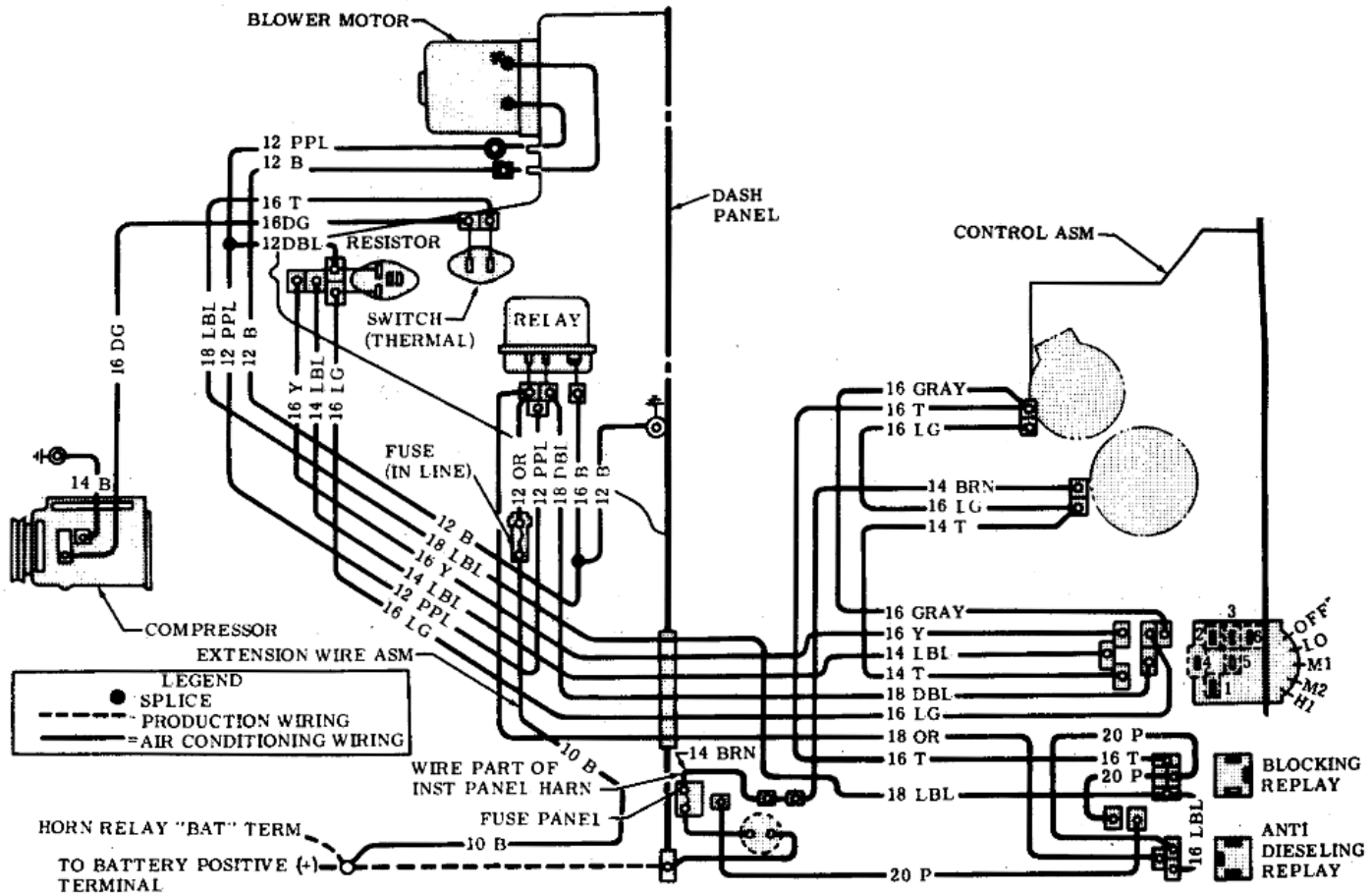
1971-72 Chevelle/El Camino/Monte Carlo A/C & Heater Wiring Diagram
