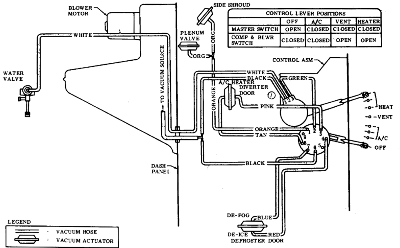
1971-72 Chevelle/El Camino/Monte Carlo A/C & Heater Vacuum Diagram
