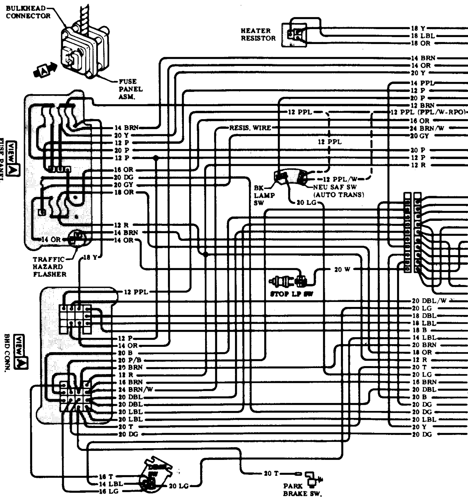
69 CAMARO .. FUSE PANEL
