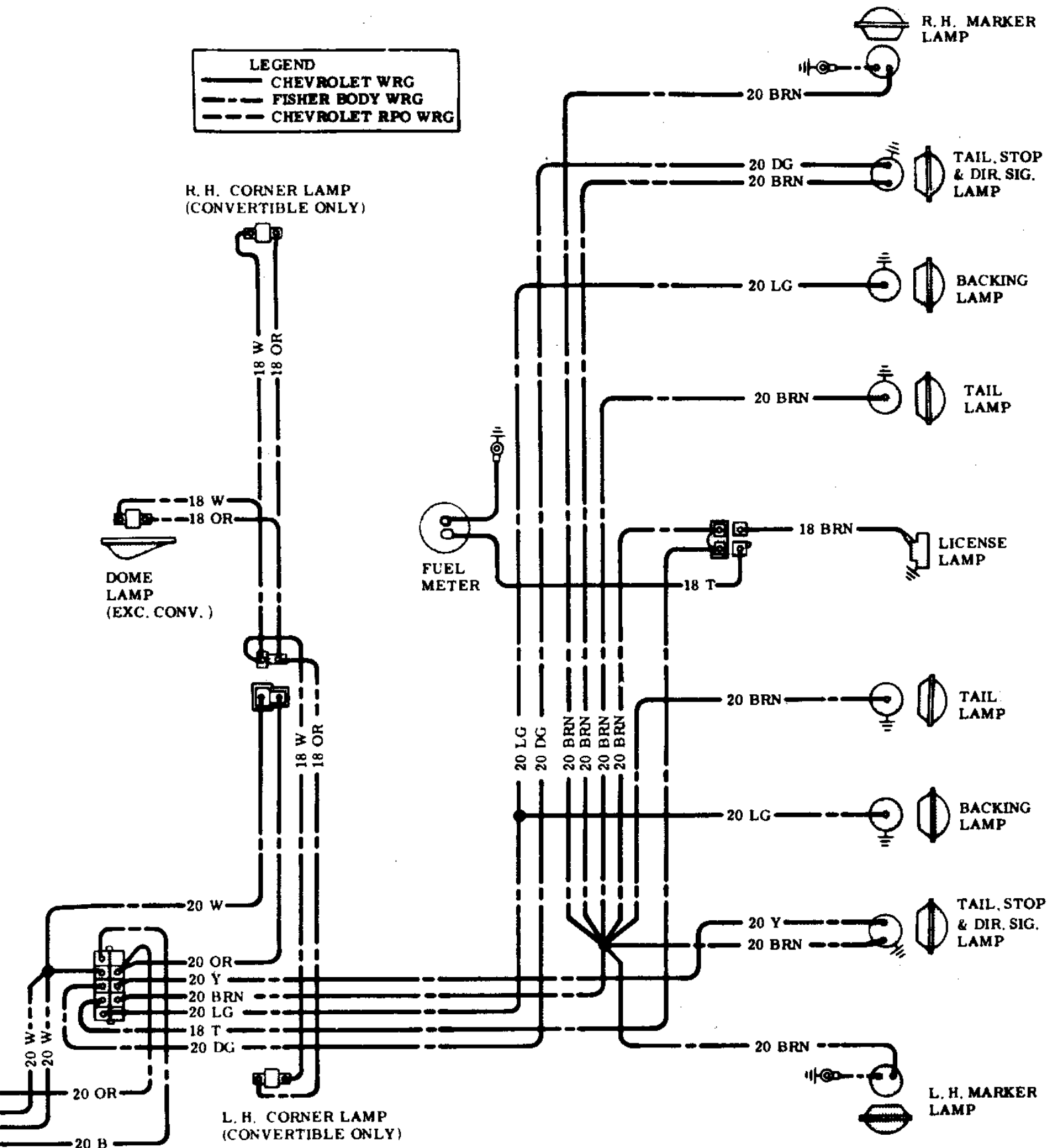
69 CAMARO .. BODY & REAR LIGHTING
