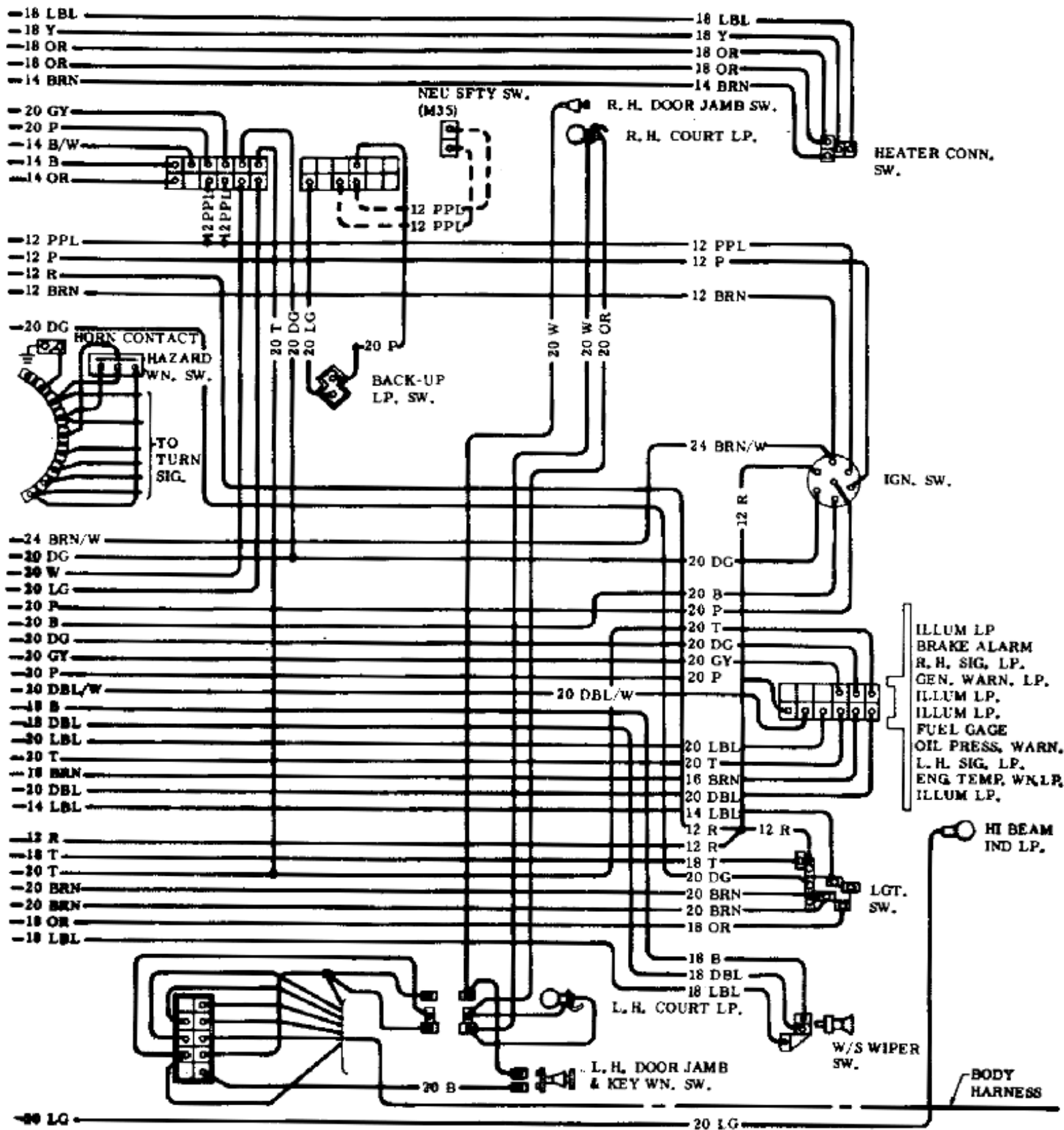
68 CAMARO .. INSTRUMENT PANEL & CLUSTER
