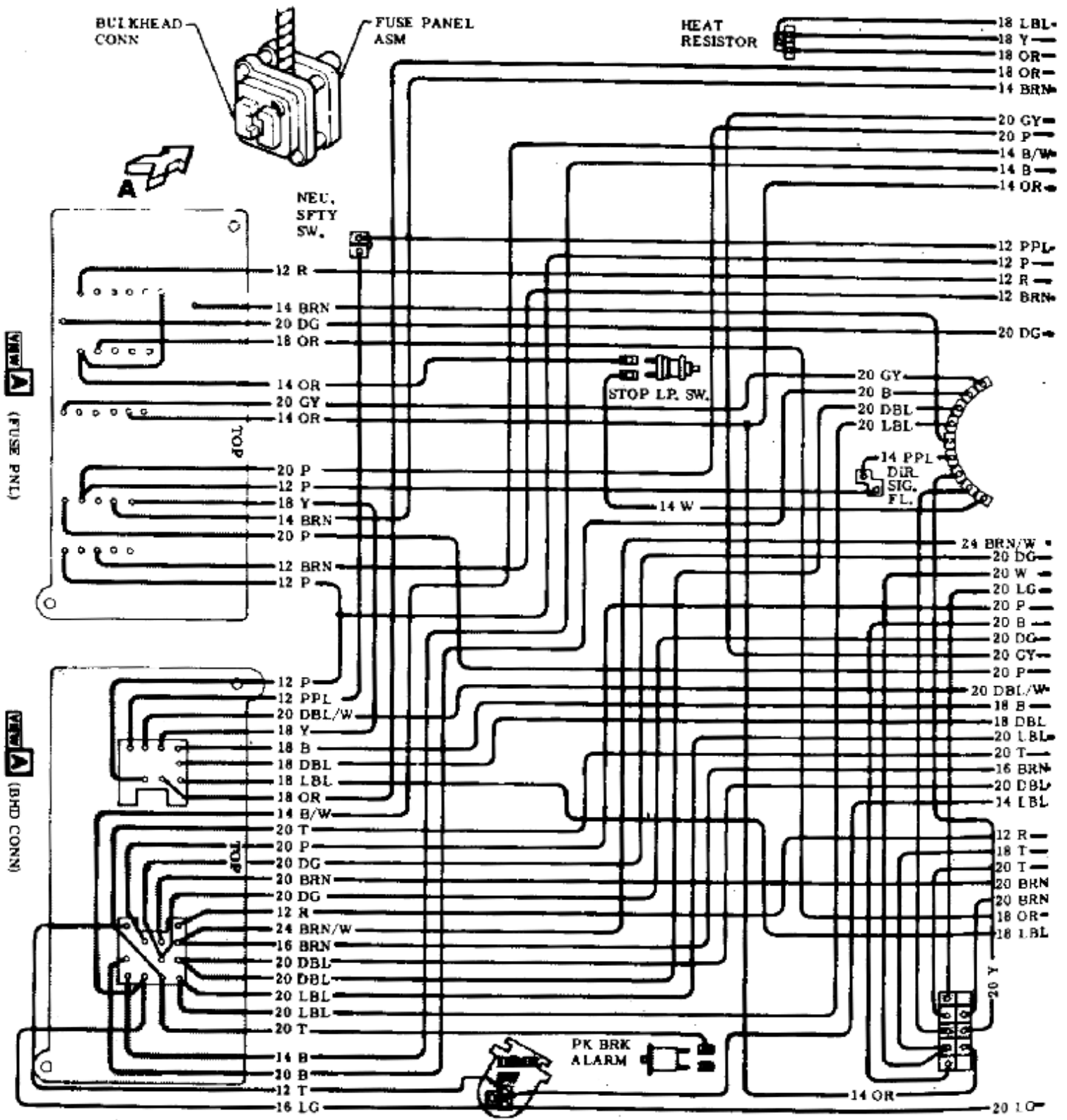
68 CAMARO .. FUSE PANEL
