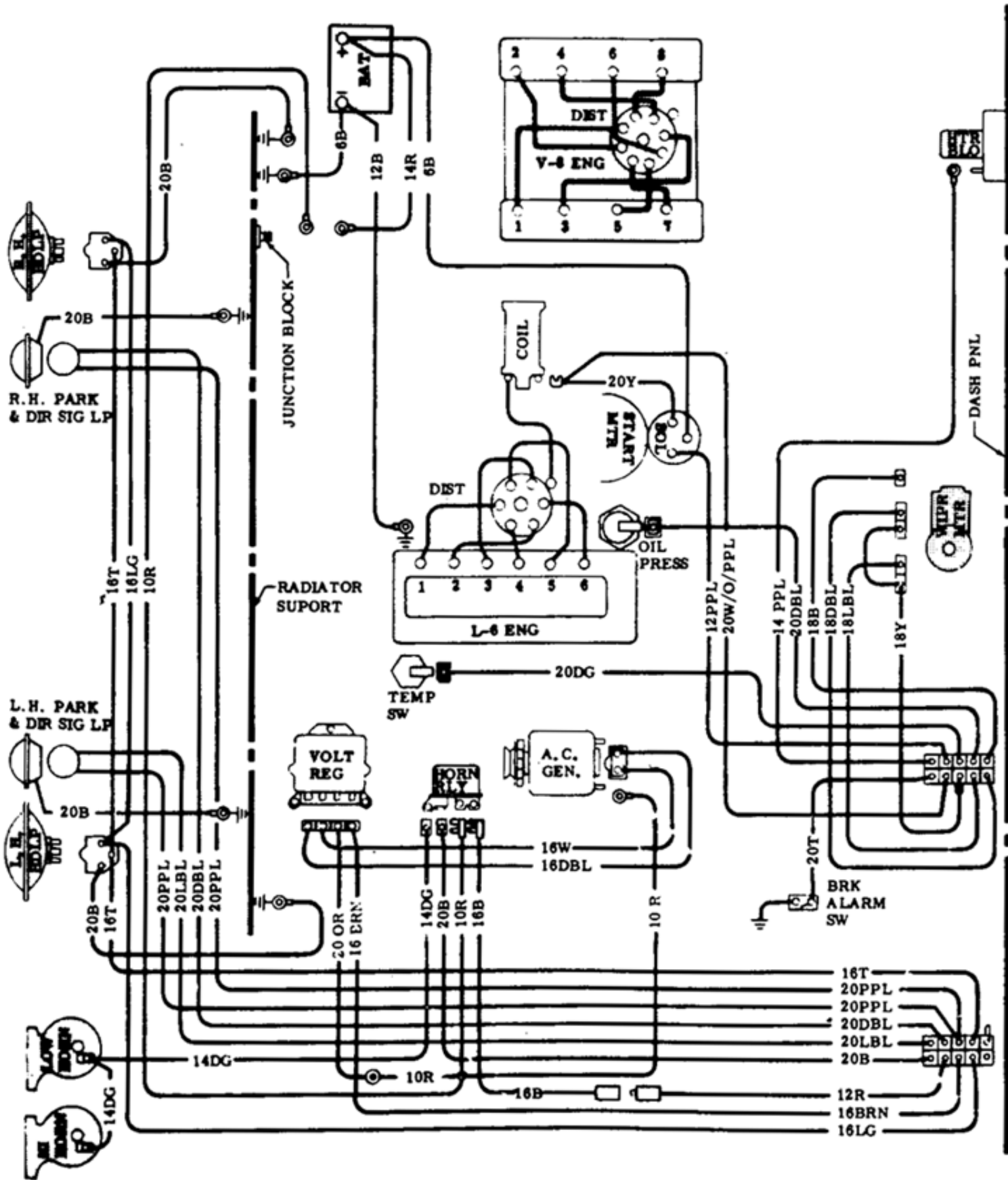
67 CAMARO .. FRONT LIGHTING & ENGINE
