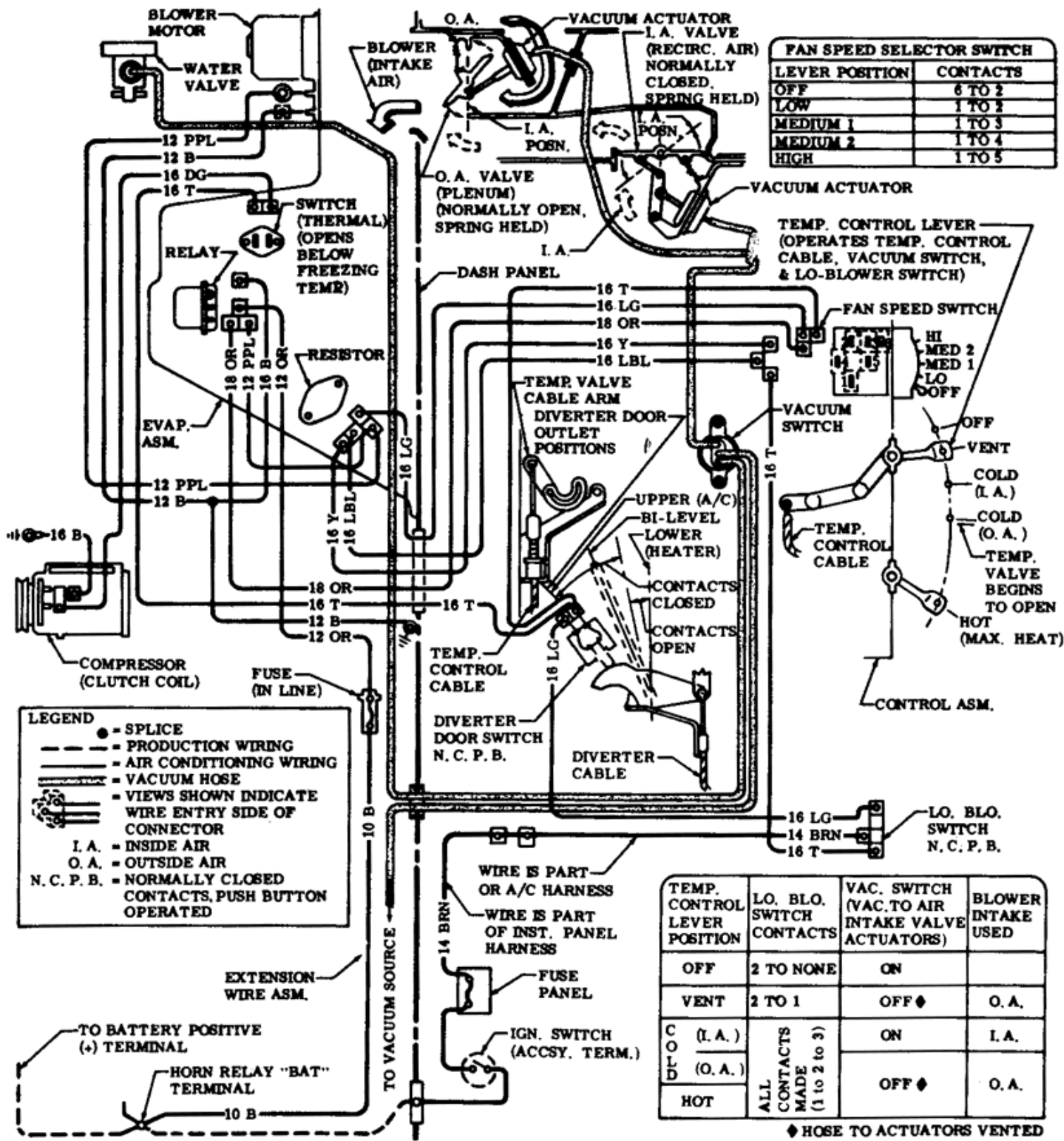
Air Conditioning & Heater Circuits . . 1969
